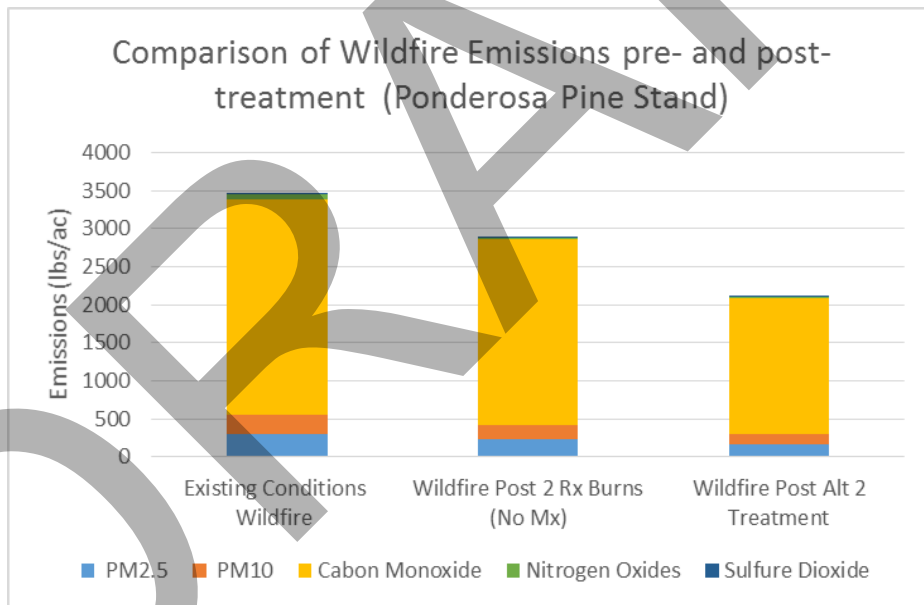
Figure 36: Alternative 2 comparison of wildfire emissions pre- and post- treatments
